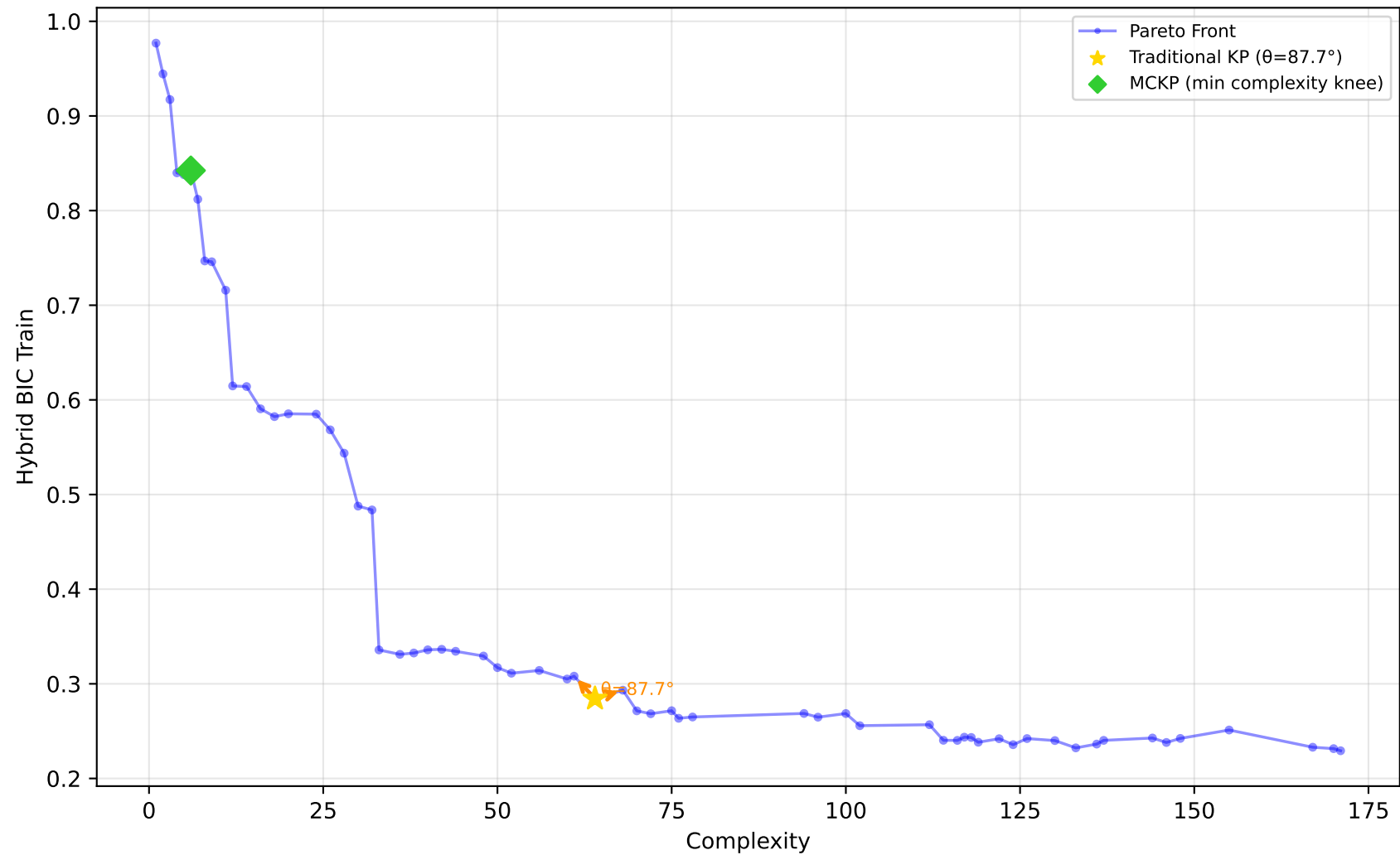
584_fri_c4_500_25 - Run 6 - MVP - Hybrid BIC Train \lambda_1=0.00 , \lambda_2=0.00 , \lambda_3=0.00 | Difficulty: 1.00 | Method: hmr
