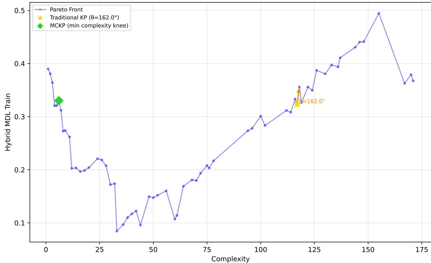
584_fri_c4_500_25 - Run 6 - MVP - Hybrid MDL Train \lambda_1=0.10, \lambda_2=0.00, \lambda_3=0.00 | Difficulty: 1.00 | Method: hmr
