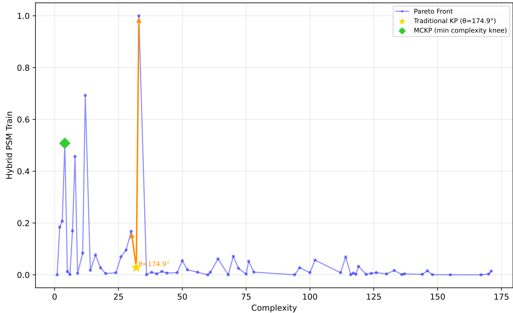
584_fri_c4_500_25 - Run 6 - MVP - Hybrid PSM Train \lambda_1=0.00, \lambda_2=0.00, \lambda_3=0.00 | Difficulty: 1.00 | Method: hmr
