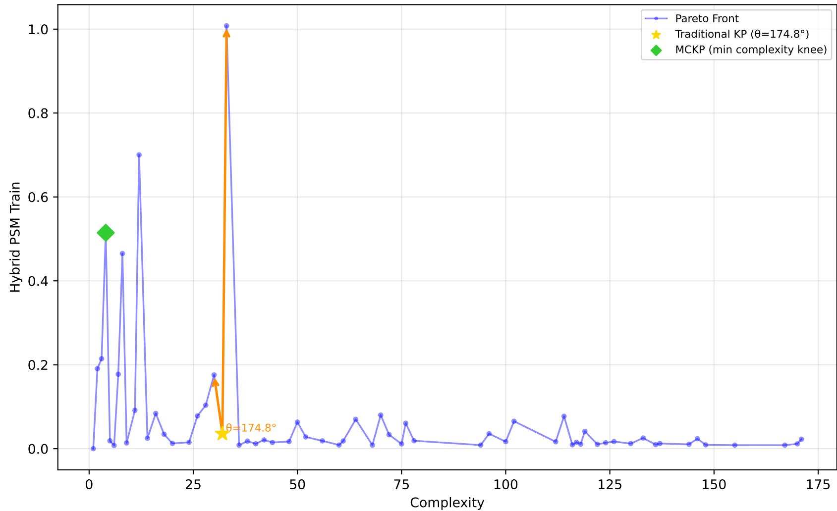
584_fri_c4_500_25 - Run 6 - MVP - Hybrid PSM Train \lambda_1=0.10, \lambda_2=0.00, \lambda_3=0.00 | Difficulty: 1.00 | Method: hmr
