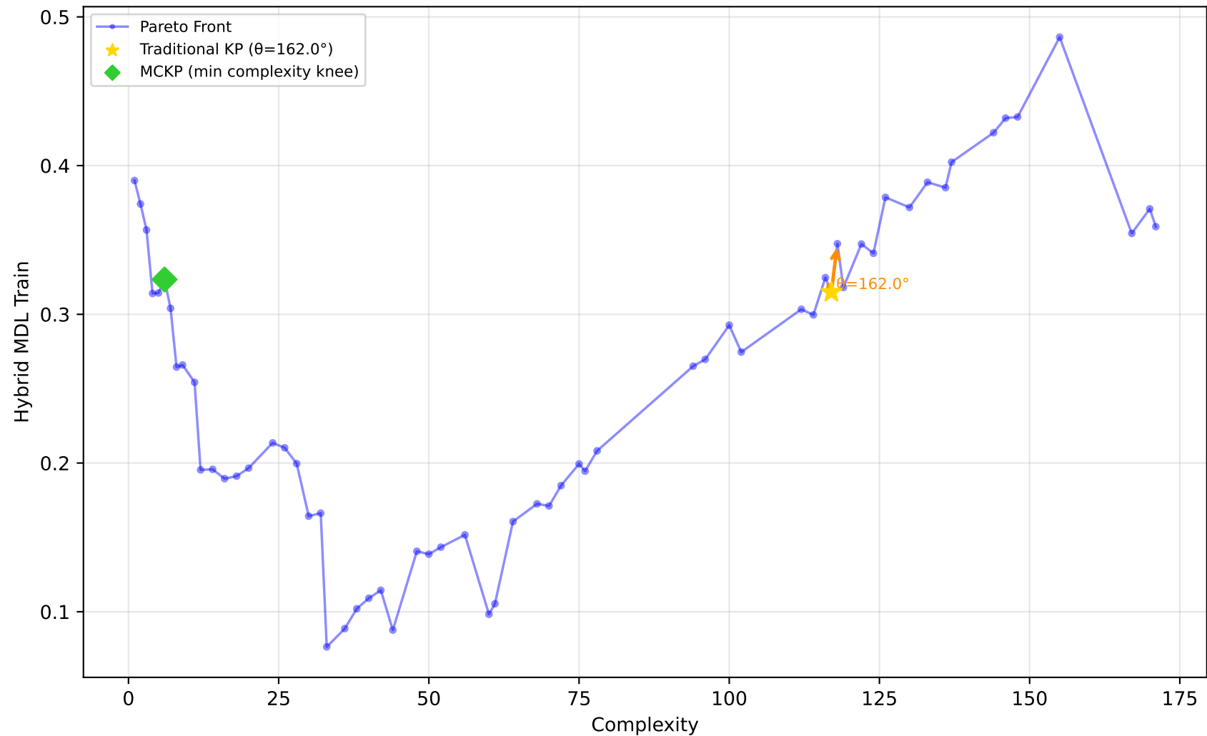
584_fri_c4_500_25 - Run 6 - SVP - Hybrid MDL Train \lambda_1=0.00, \lambda_2=0.00, \lambda_3=0.00 | Difficulty: 1.00 | Method: hmr
