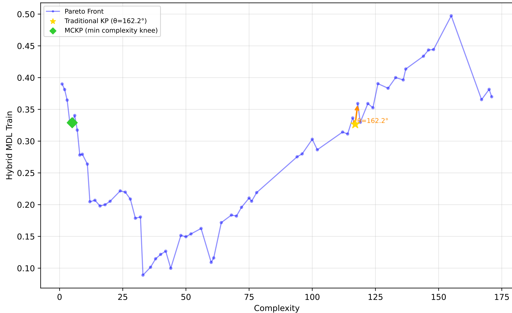
584_fri_c4_500_25 - Run 6 - SVP - Hybrid MDL Train \lambda_1=0.10 , \lambda_2=0.40 , \lambda_3=0.00 | Difficulty: 1.00 | Method: hmr
