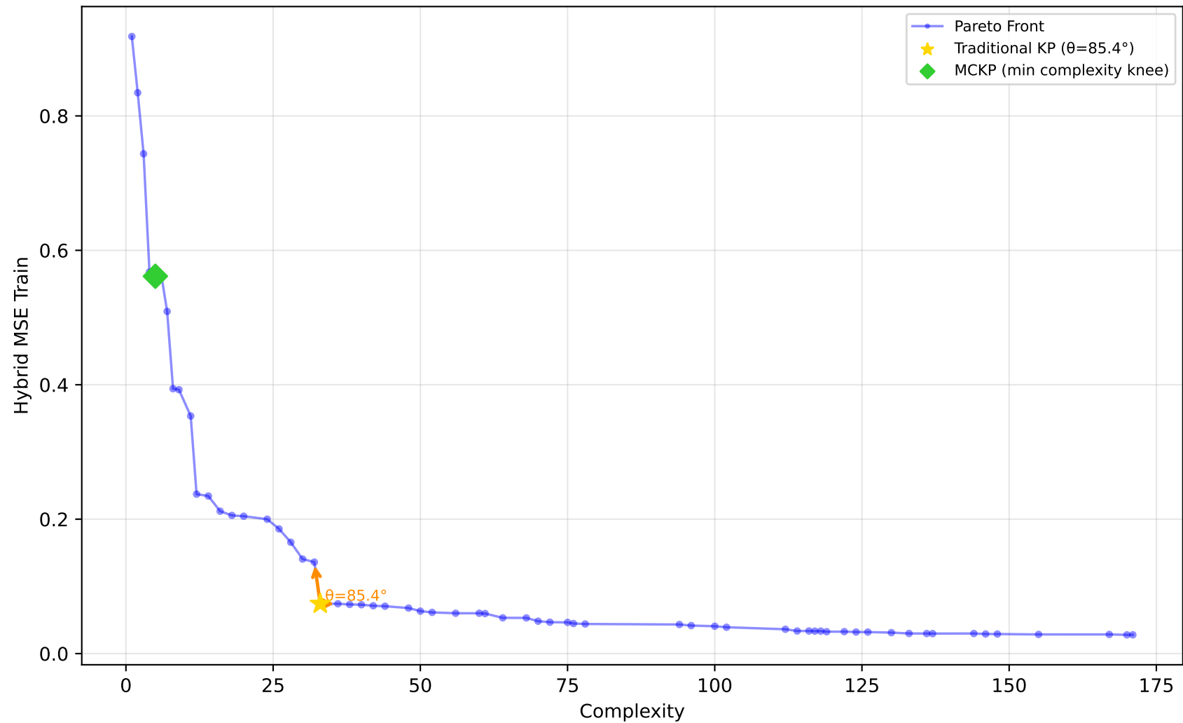
584_fri_c4_500_25 - Run 6 - SVP - Hybrid MSE Train \lambda_1=0.10, \lambda_2=0.40, \lambda_3=0.00 | Difficulty: 1.00 | Method: hmr
