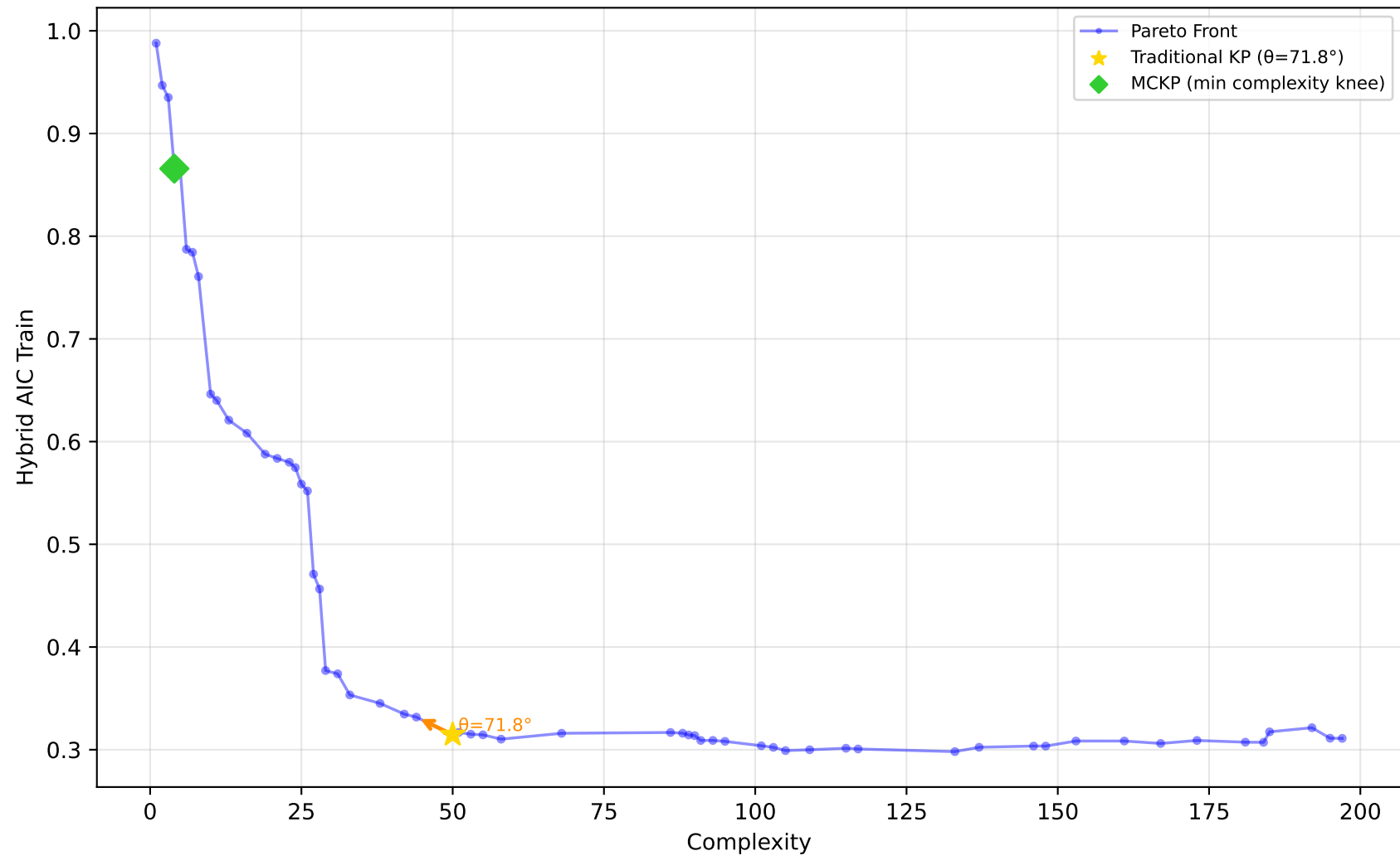
584_fri_c4_500_25 - Run 7 - MVP - Hybrid AIC Train \lambda_1=0.00, \lambda_2=0.00, \lambda_3=0.00 | Difficulty: 1.00 | Method: hmr
