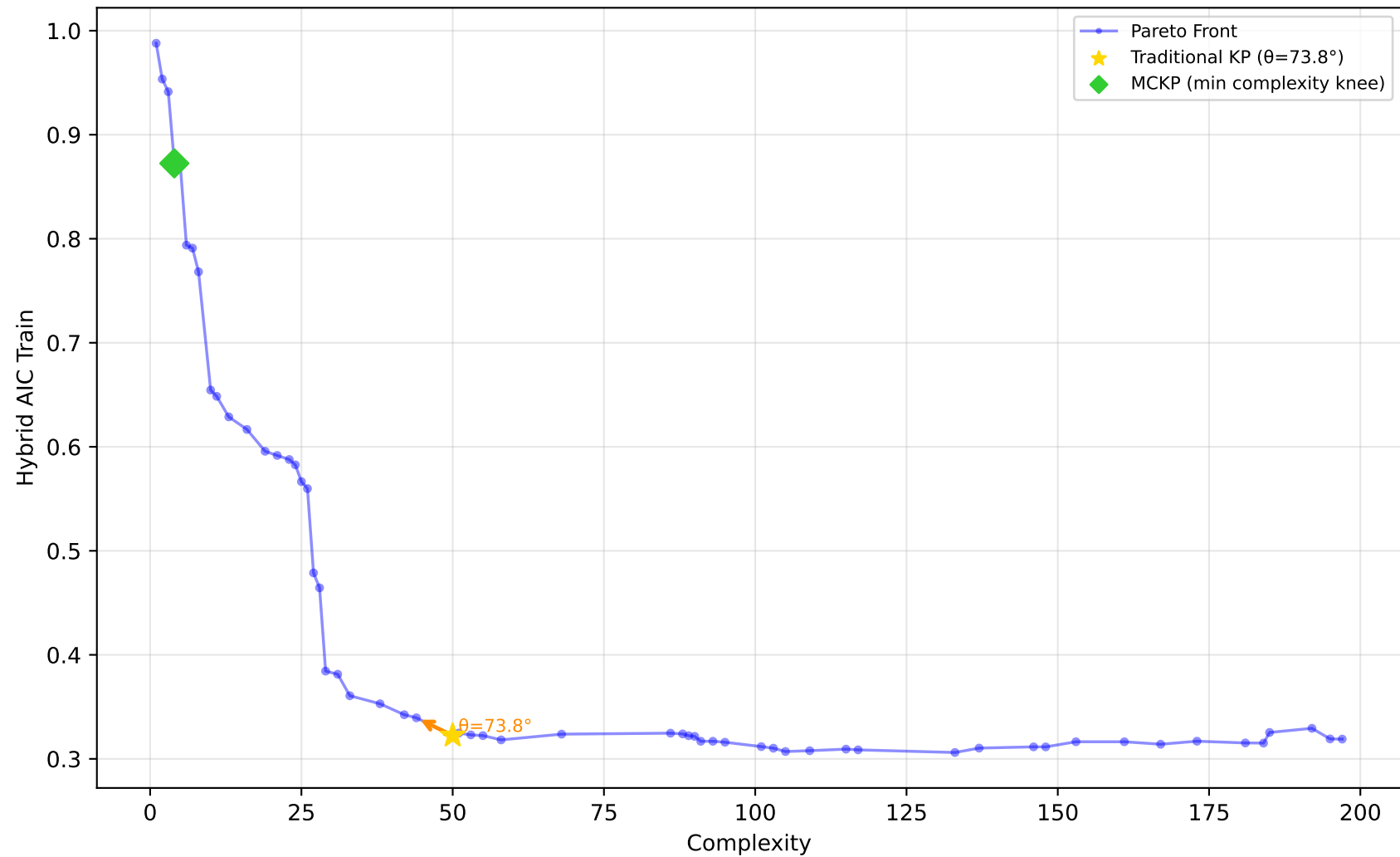
584_fri_c4_500_25 - Run 7 - MVP - Hybrid AIC Train \lambda_1=0.10, \lambda_2=0.00, \lambda_3=0.00 | Difficulty: 1.00 | Method: hmr
