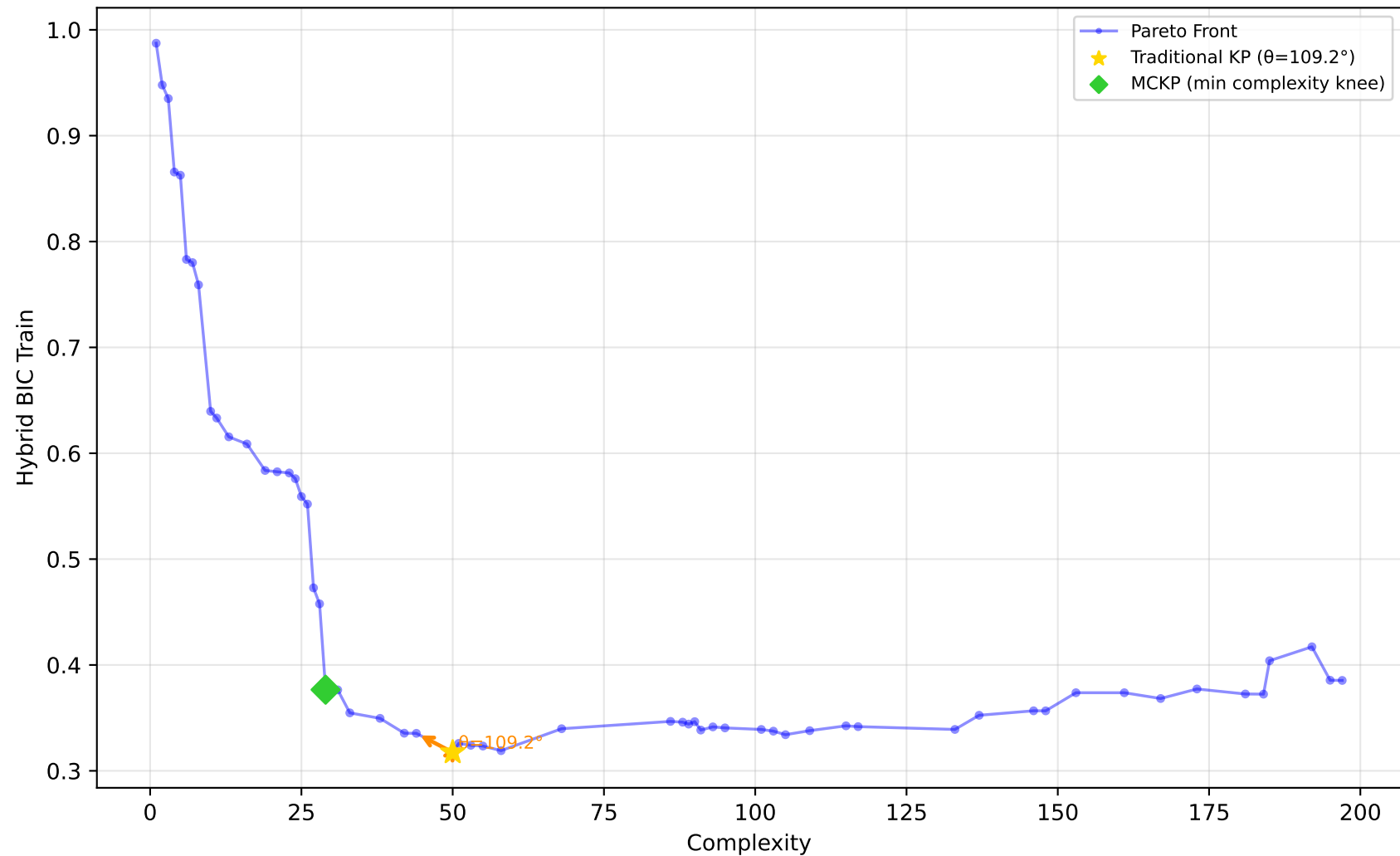
584_fri_c4_500_25 - Run 7 - MVP - Hybrid BIC Train \lambda_1=0.10, \lambda_2=0.00, \lambda_3=0.00 | Difficulty: 1.00 | Method: hmr
