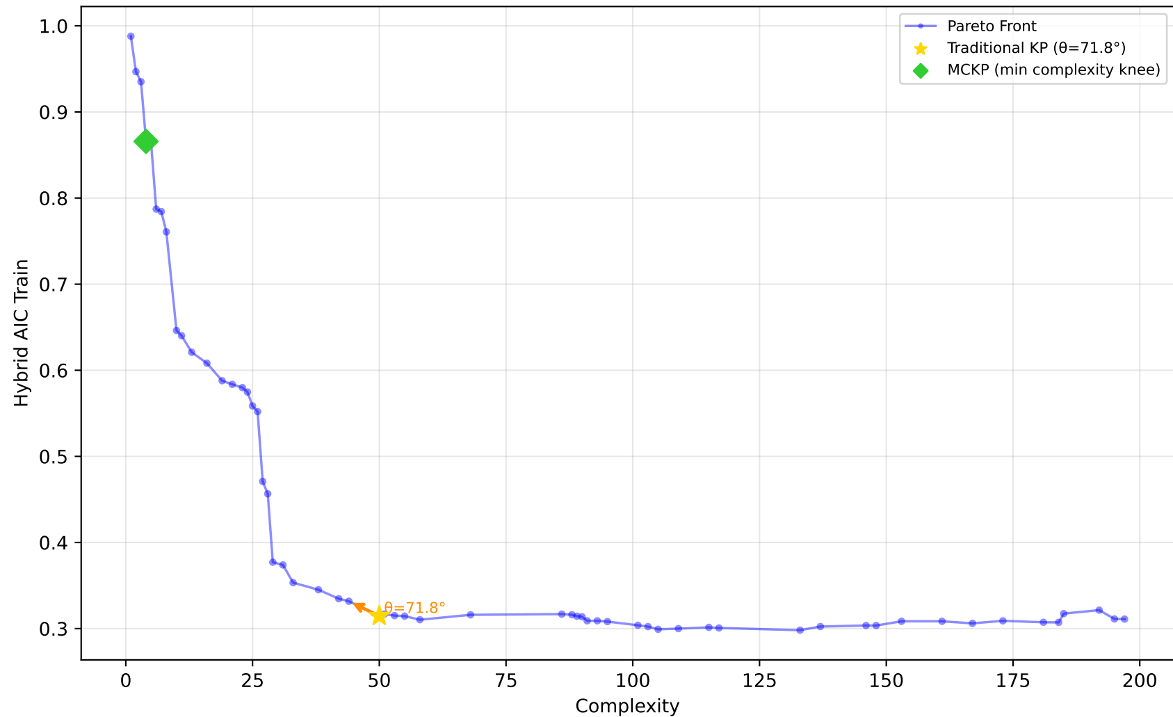
584_fri_c4_500_25 - Run 7 - SVP - Hybrid AIC Train \lambda_1=0.00, \lambda_2=0.00, \lambda_3=0.00 | Difficulty: 1.00 | Method: hmr
