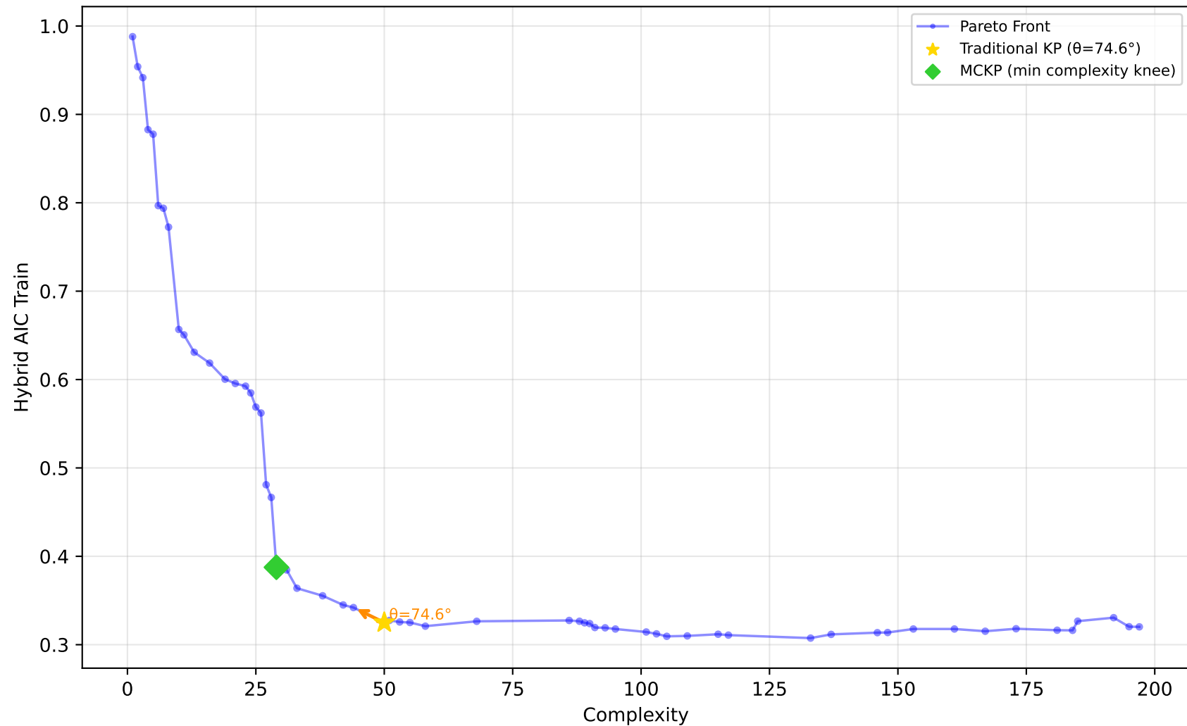
584_fri_c4_500_25 - Run 7 - SVP - Hybrid AIC Train \lambda_1=0.10, \lambda_2=0.40, \lambda_3=0.00 | Difficulty: 1.00 | Method: hmr
