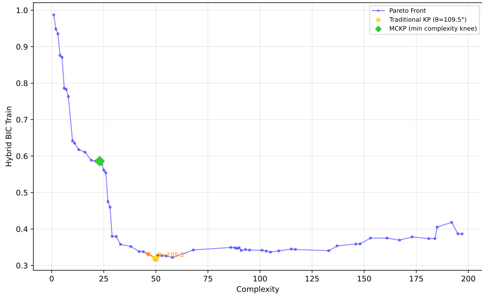
584_fri_c4_500_25 - Run 7 - SVP - Hybrid BIC Train \lambda_1=0.10, \lambda_2=0.40, \lambda_3=0.00 | Difficulty: 1.00 | Method: hmr
