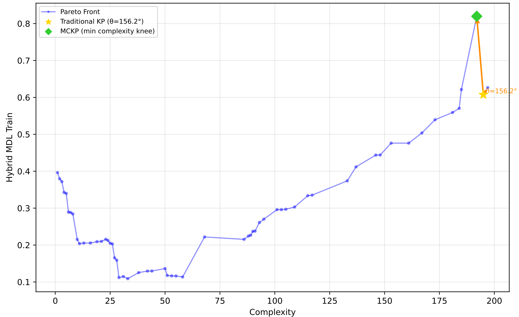
584_fri_c4_500_25 - Run 7 - SVP - Hybrid MDL Train \lambda_1=0.10, \lambda_2=0.40, \lambda_3=0.00 | Difficulty: 1.00 | Method: hmr
