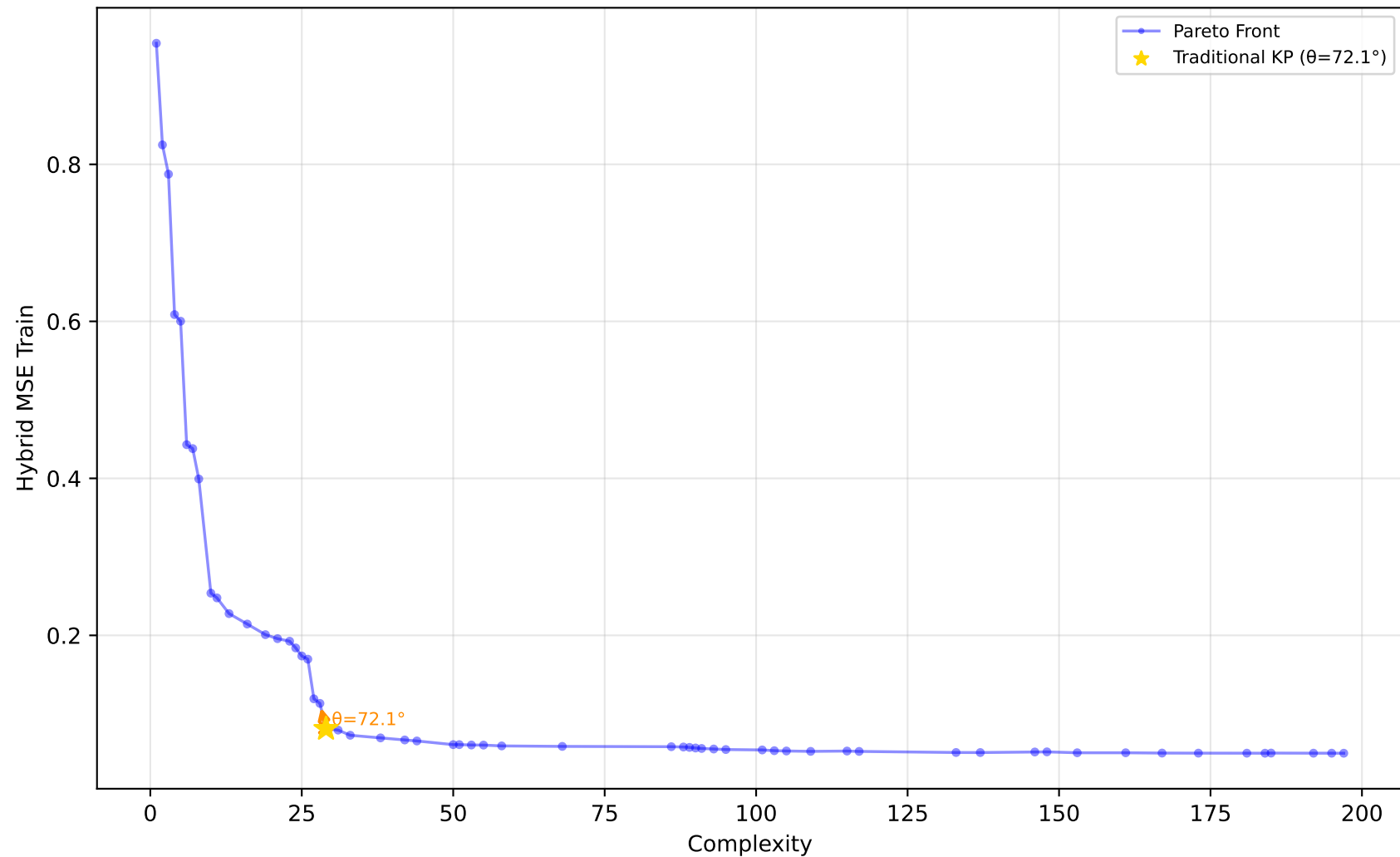
584_fri_c4_500_25 - Run 7 - SVP - Hybrid MSE Train \lambda_1=0.10, \lambda_2=0.40, \lambda_3=0.00 | Difficulty: 1.00 | Method: hmr
