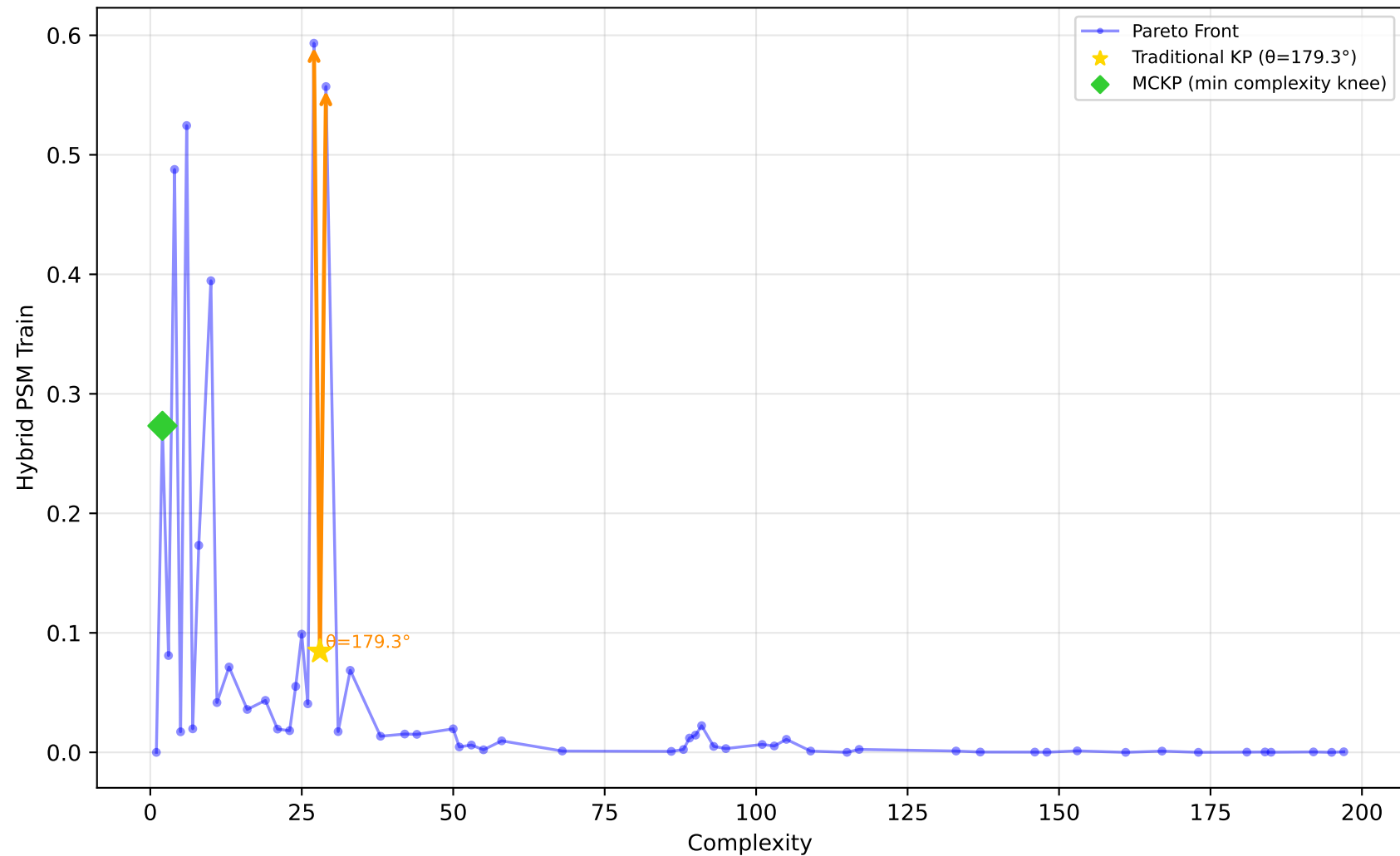
584_fri_c4_500_25 - Run 7 - SVP - Hybrid PSM Train \lambda_1=0.00, \lambda_2=0.00, \lambda_3=0.00 | Difficulty: 1.00 | Method: hmr
