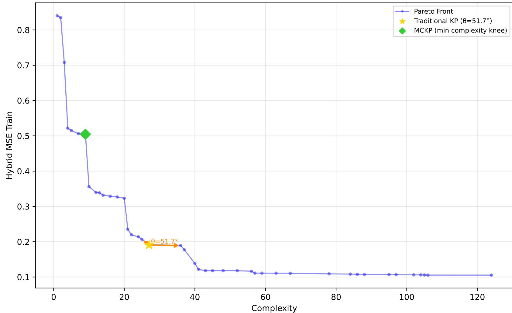
584_fri_c4_500_25 - Run 8 - MVP - Hybrid MSE Train \lambda_1=0.10, \lambda_2=0.00, \lambda_3=0.00 | Difficulty: 1.00 | Method: hmr
