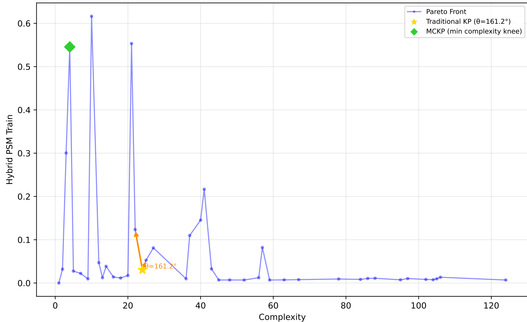
584_fri_c4_500_25 - Run 8 - MVP - Hybrid PSM Train \lambda_1=0.10, \lambda_2=0.00, \lambda_3=0.00 | Difficulty: 1.00 | Method: hmr
