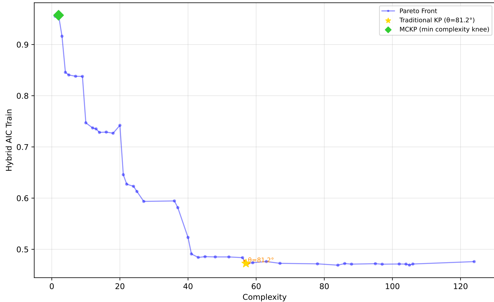
584_fri_c4_500_25 - Run 8 - SVP - Hybrid AIC Train \lambda_1=0.10, \lambda_2=0.40, \lambda_3=0.00 | Difficulty: 1.00 | Method: hmr
