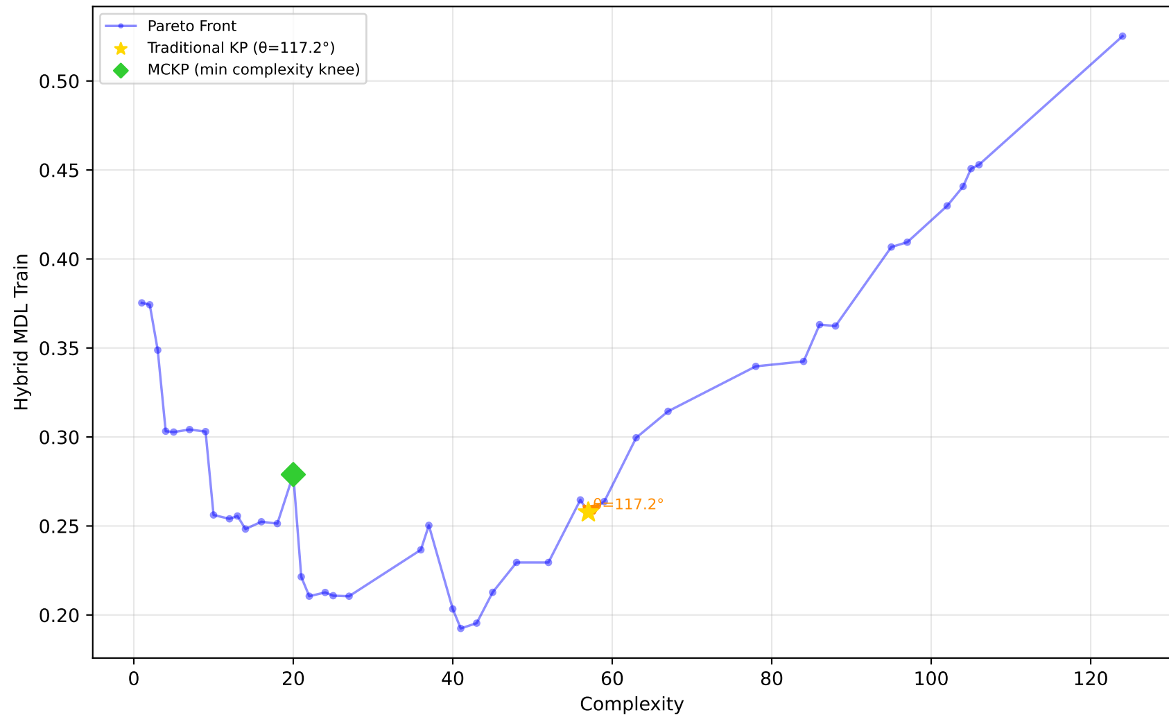
584_fri_c4_500_25 - Run 8 - SVP - Hybrid MDL Train \lambda_1=0.00 , \lambda_2=0.00 , \lambda_3=0.00 | Difficulty: 1.00 | Method: hmr
