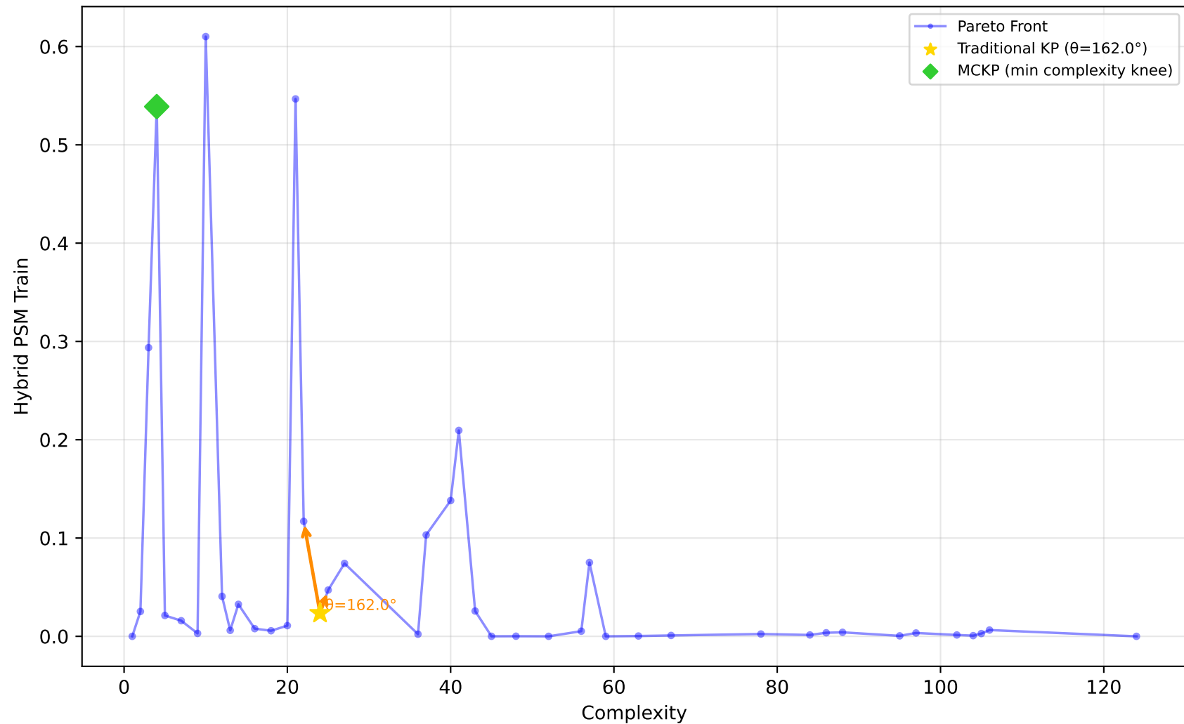
584_fri_c4_500_25 - Run 8 - SVP - Hybrid PSM Train \lambda_1=0.00 , \lambda_2=0.00 , \lambda_3=0.00 | Difficulty: 1.00 | Method: hmr
