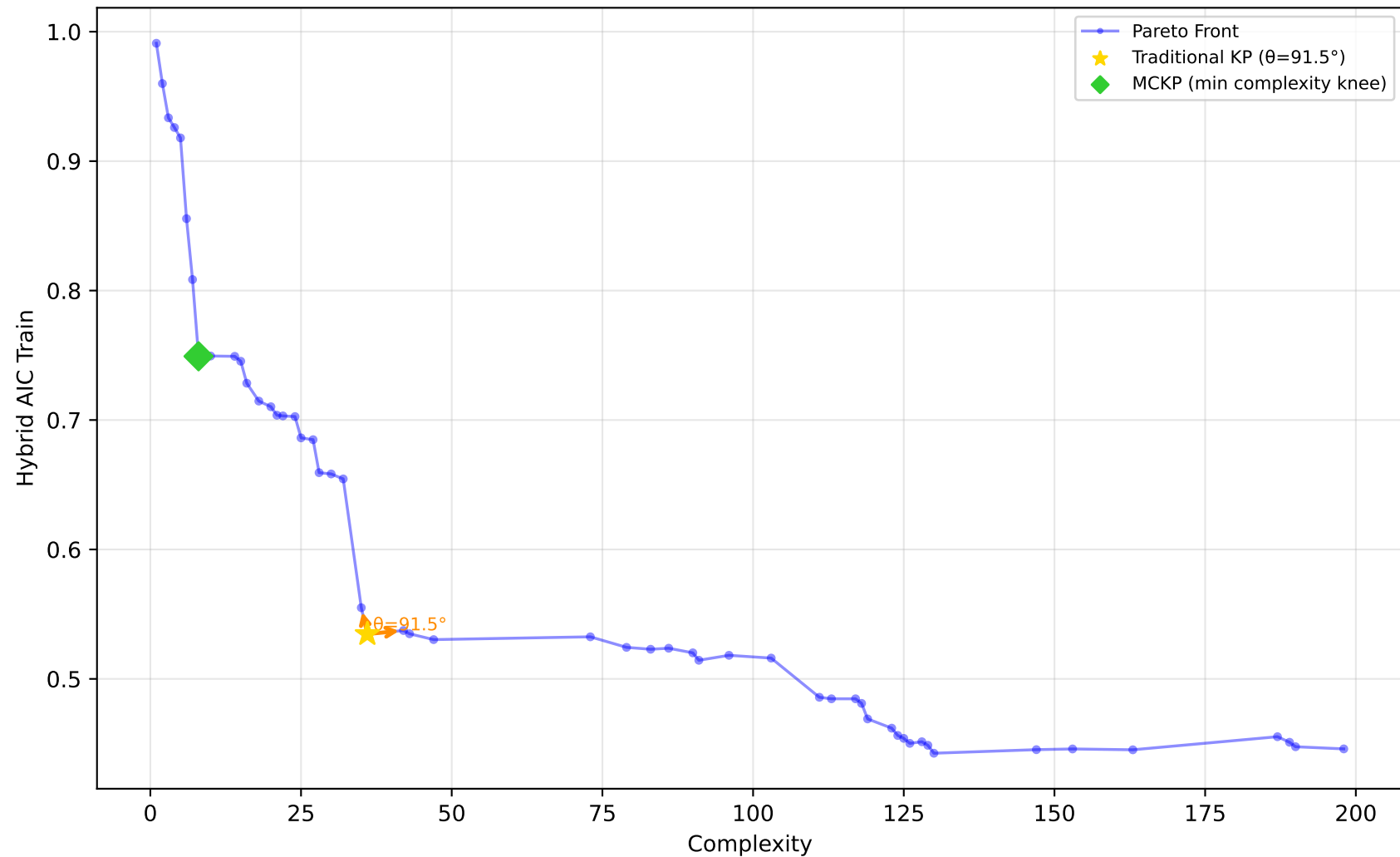
584_fri_c4_500_25 - Run 9 - MVP - Hybrid AIC Train \lambda_1=0.00, \lambda_2=0.00, \lambda_3=0.00 | Difficulty: 1.00 | Method: hmr
