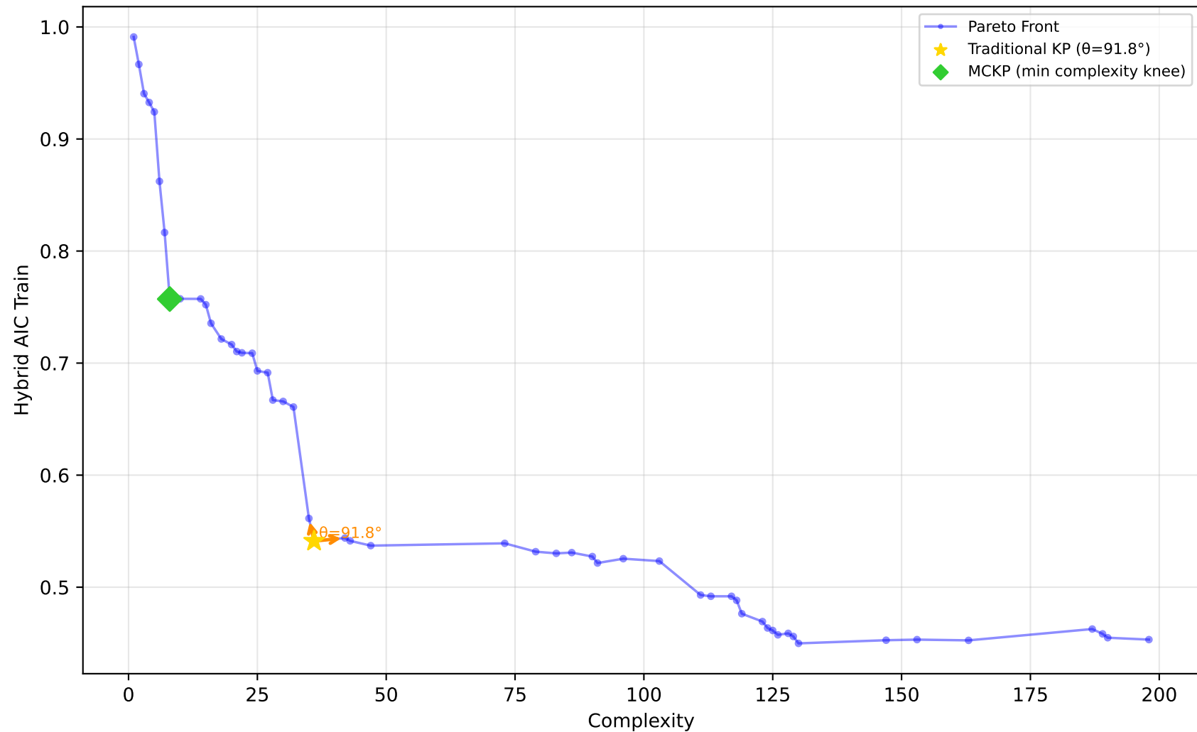
584_fri_c4_500_25 - Run 9 - MVP - Hybrid AIC Train \lambda_1=0.10, \lambda_2=0.00, \lambda_3=0.00 | Difficulty: 1.00 | Method: hmr
