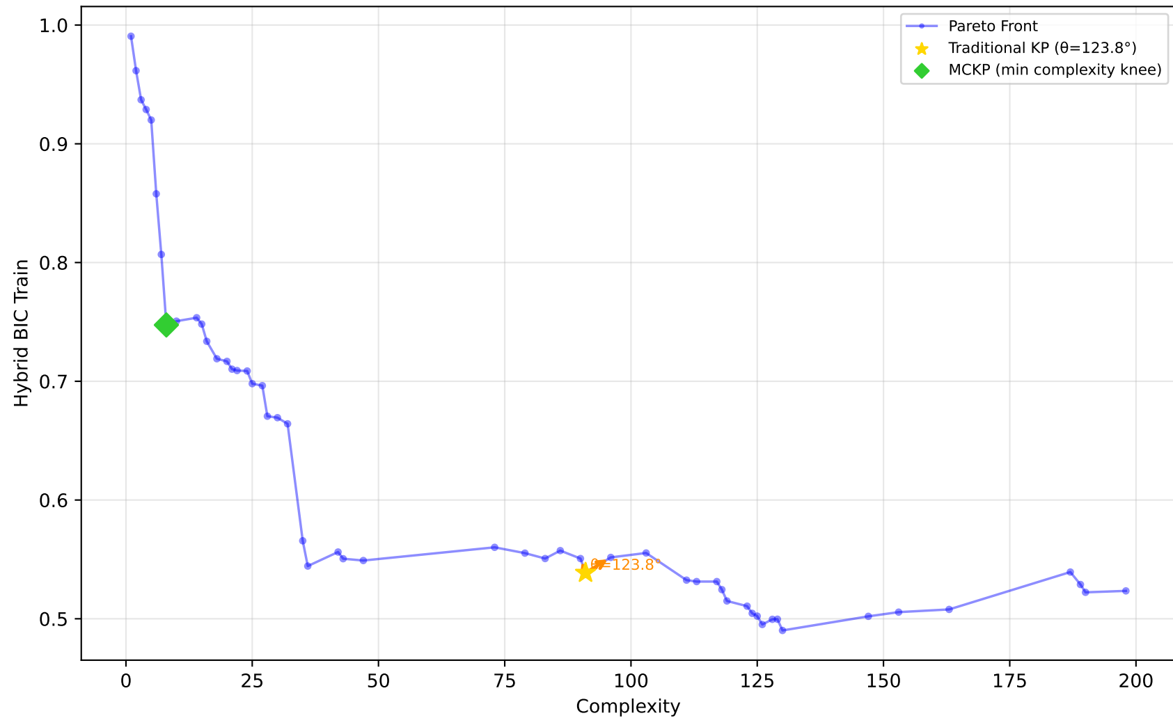
584_fri_c4_500_25 - Run 9 - MVP - Hybrid BIC Train \lambda_1=0.10, \lambda_2=0.00, \lambda_3=0.00 | Difficulty: 1.00 | Method: hmr
