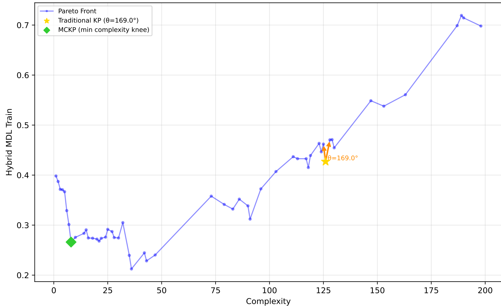
584_fri_c4_500_25 - Run 9 - MVP - Hybrid MDL Train \lambda_1=0.10, \lambda_2=0.00, \lambda_3=0.00 | Difficulty: 1.00 | Method: hmr
