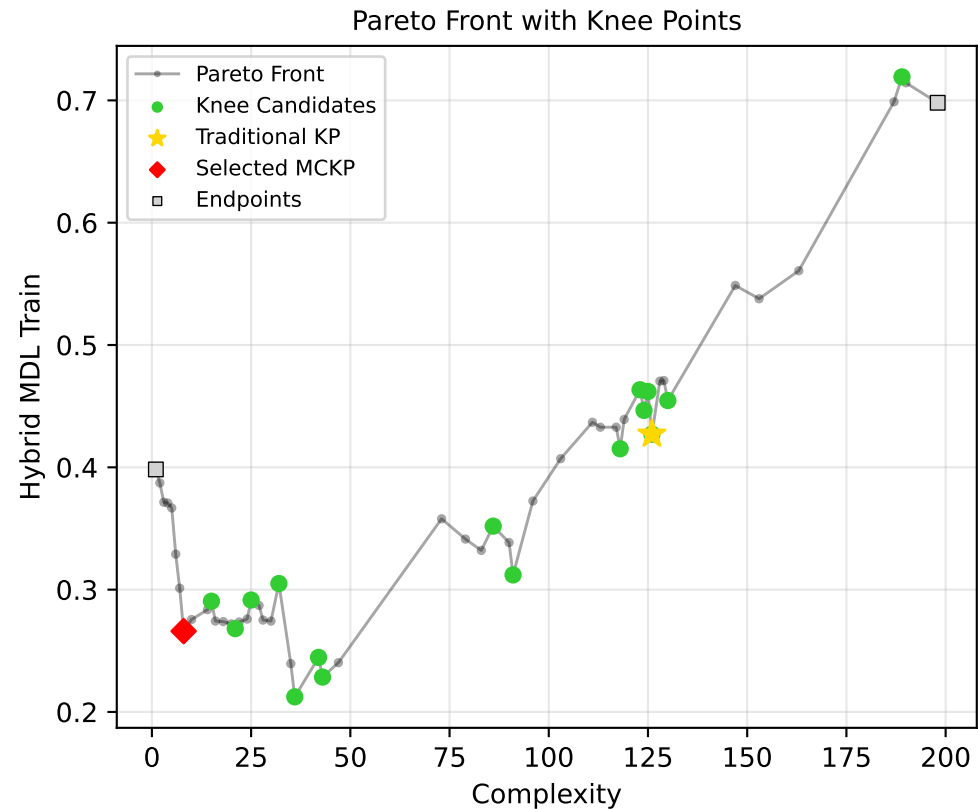
584_fri_c4_500_25 - Run 9 - MVP - Hybrid MDL Train - Clustering Threshold \lambda_1=0.10, \lambda_2=0.00, \lambda_3=0.00 | Difficulty: 1.00
