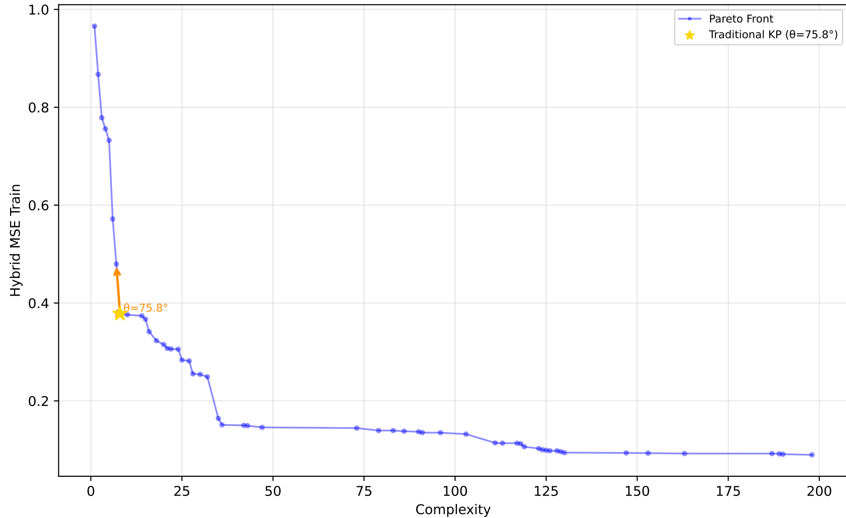
584_fri_c4_500_25 - Run 9 - MVP - Hybrid MSE Train \lambda_1=0.10, \lambda_2=0.00, \lambda_3=0.00 | Difficulty: 1.00 | Method: hmr
