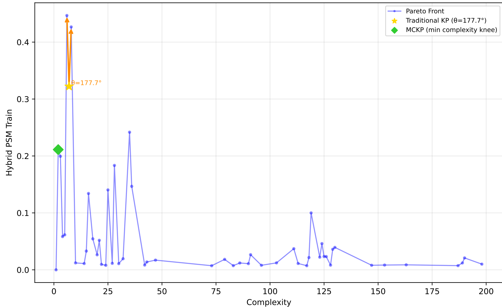
584_fri_c4_500_25 - Run 9 - MVP - Hybrid PSM Train \lambda_1=0.10, \lambda_2=0.00, \lambda_3=0.00 | Difficulty: 1.00 | Method: hmr
