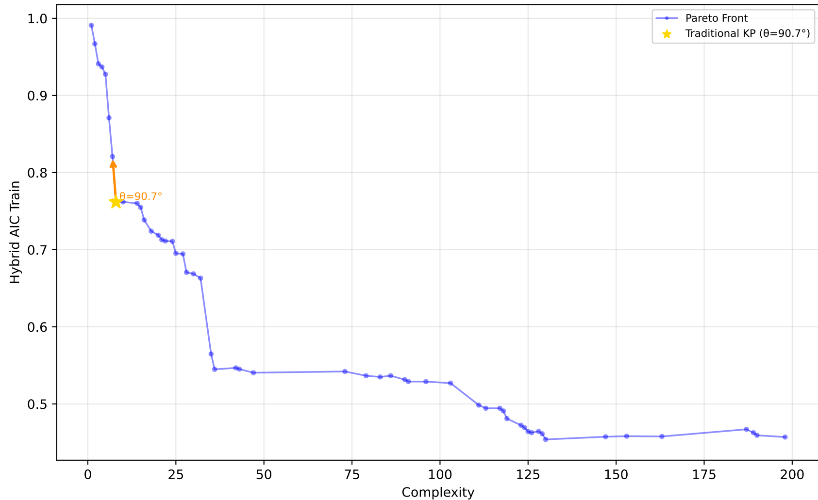
584_fri_c4_500_25 - Run 9 - SVP - Hybrid AIC Train \lambda_1=0.10, \lambda_2=0.40, \lambda_3=0.00 | Difficulty: 1.00 | Method: hmr
