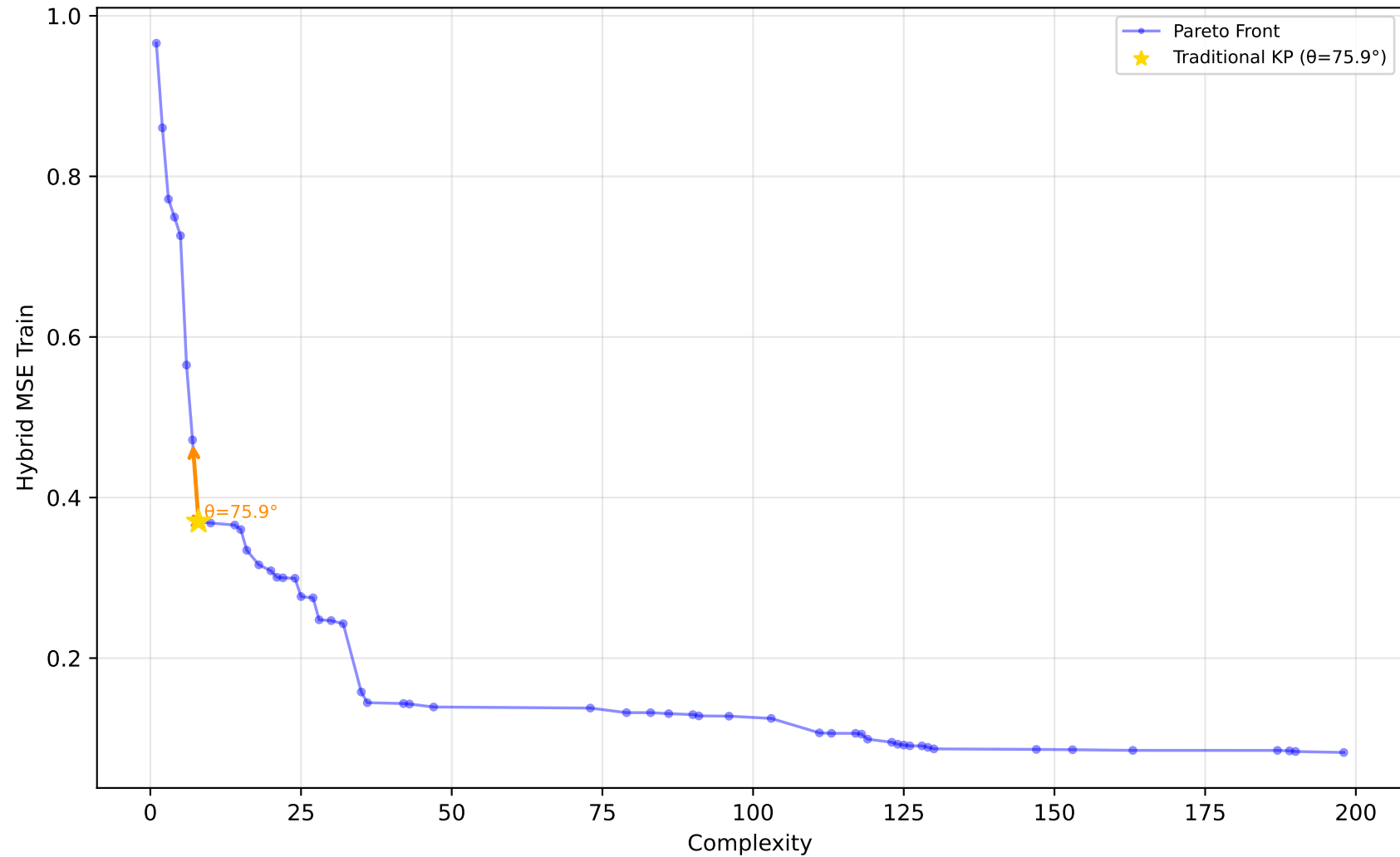
584_fri_c4_500_25 - Run 9 - SVP - Hybrid MSE Train \lambda_1=0.00, \lambda_2=0.00, \lambda_3=0.00 | Difficulty: 1.00 | Method: hmr
