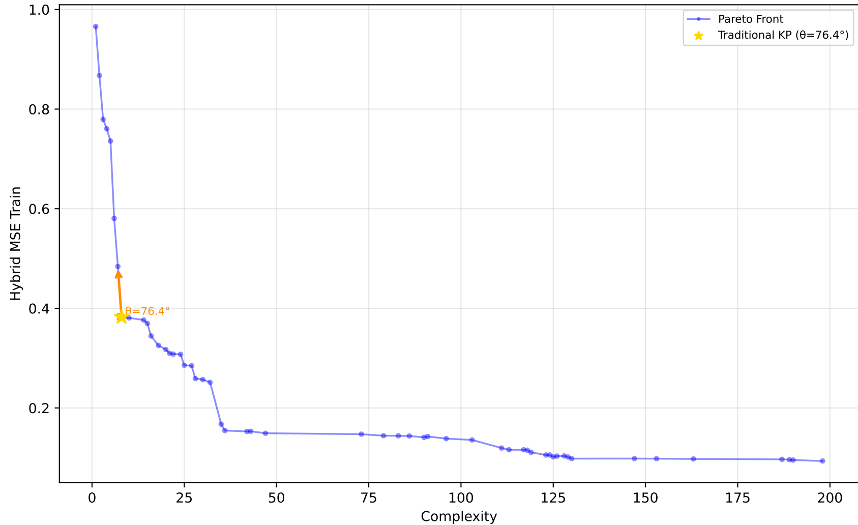
584_fri_c4_500_25 - Run 9 - SVP - Hybrid MSE Train \lambda_1=0.10, \lambda_2=0.40, \lambda_3=0.00 | Difficulty: 1.00 | Method: hmr
