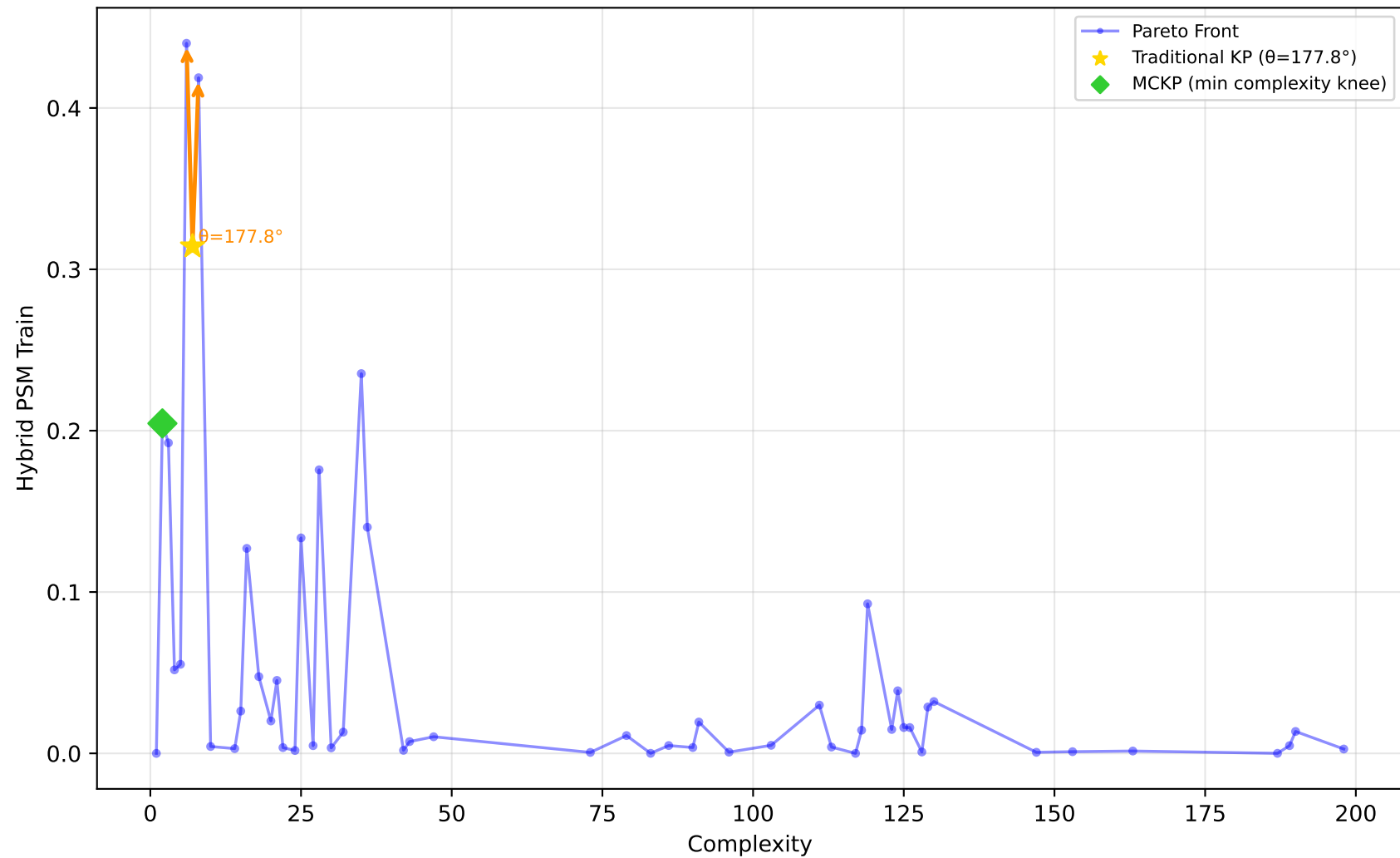
584_fri_c4_500_25 - Run 9 - SVP - Hybrid PSM Train \lambda_1=0.00, \lambda_2=0.00, \lambda_3=0.00 | Difficulty: 1.00 | Method: hmr
