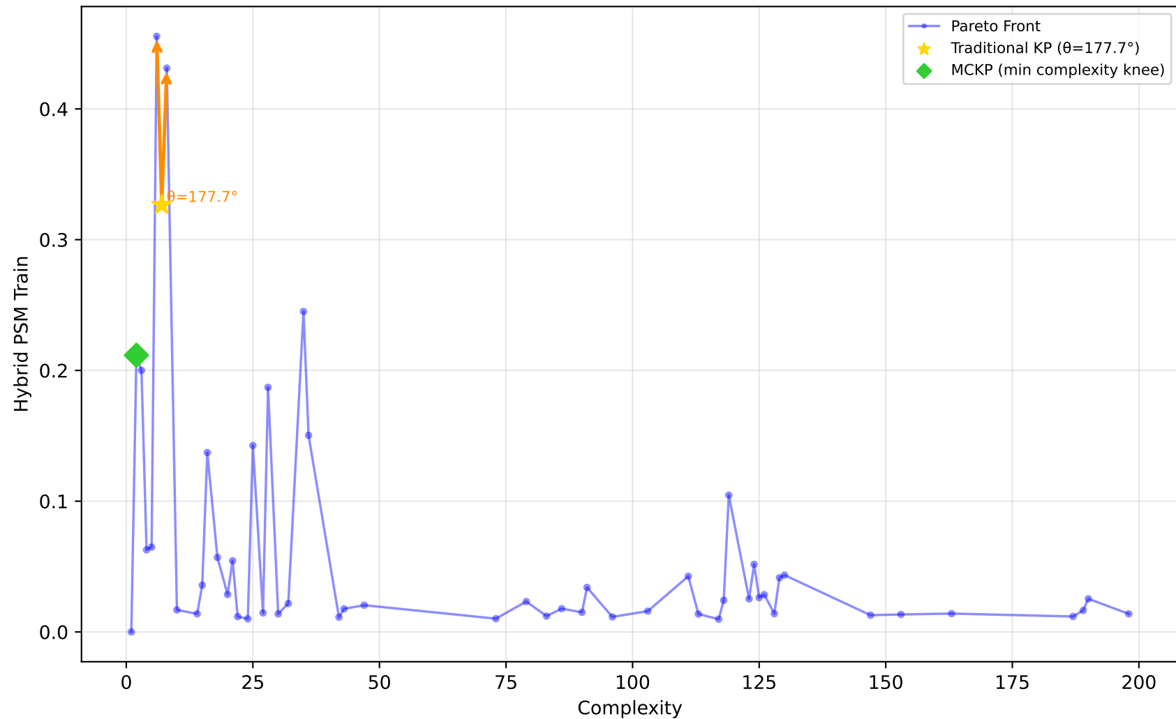
584_fri_c4_500_25 - Run 9 - SVP - Hybrid PSM Train \lambda_1=0.10, \lambda_2=0.40, \lambda_3=0.00 | Difficulty: 1.00 | Method: hmr
