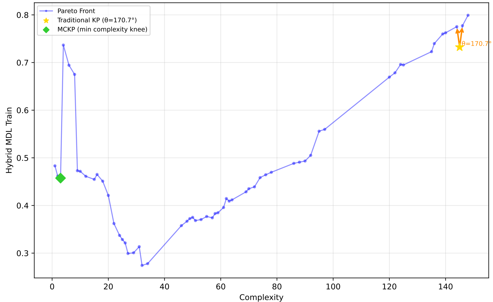
561_cpu - Run 10 - MVP - Hybrid MDL Train \lambda_1=0.50, \lambda_2=0.20, \lambda_3=0.00 | Difficulty: 1.00 | Method: hmr
