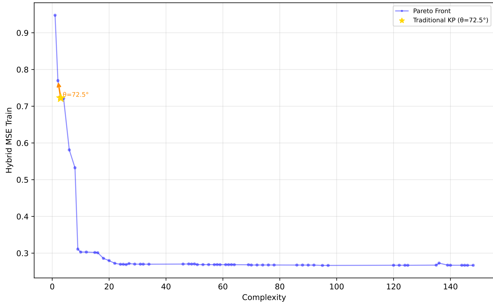
561_cpu - Run 10 - MVP - Hybrid MSE Train \lambda_1=0.50, \lambda_2=0.20, \lambda_3=0.00 | Difficulty: 1.00 | Method: hmr
