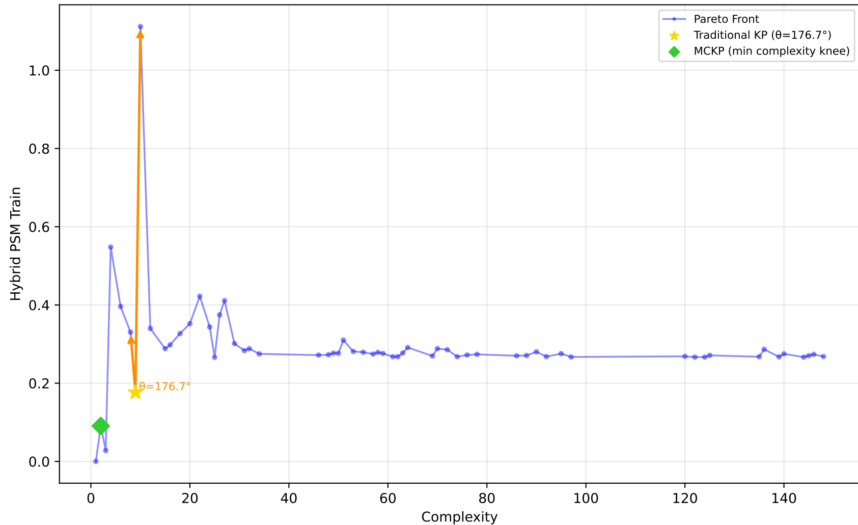
561_cpu - Run 10 - MVP - Hybrid PSM Train \lambda_1=0.50, \lambda_2=0.20, \lambda_3=0.00 | Difficulty: 1.00 | Method: hmr
