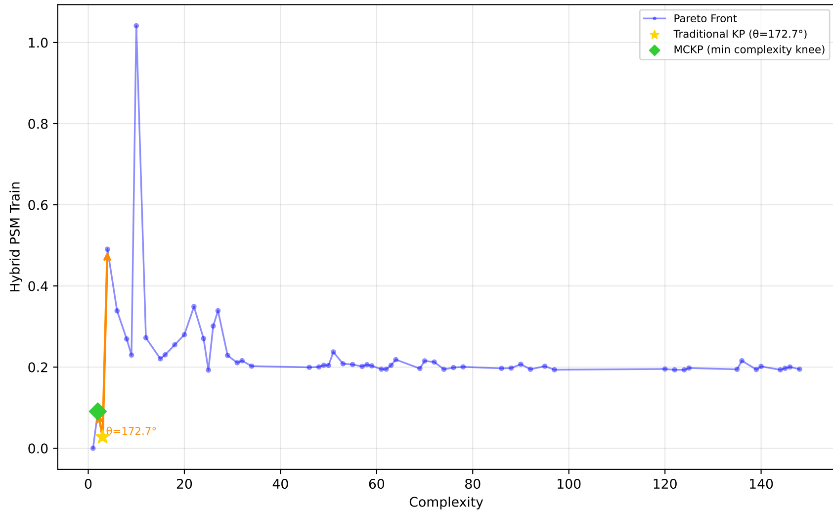
561_cpu - Run 10 - MVP - Hybrid PSM Train \lambda_1=0.70, \lambda_2=0.00, \lambda_3=0.10 | Difficulty: 1.00 | Method: hmr
