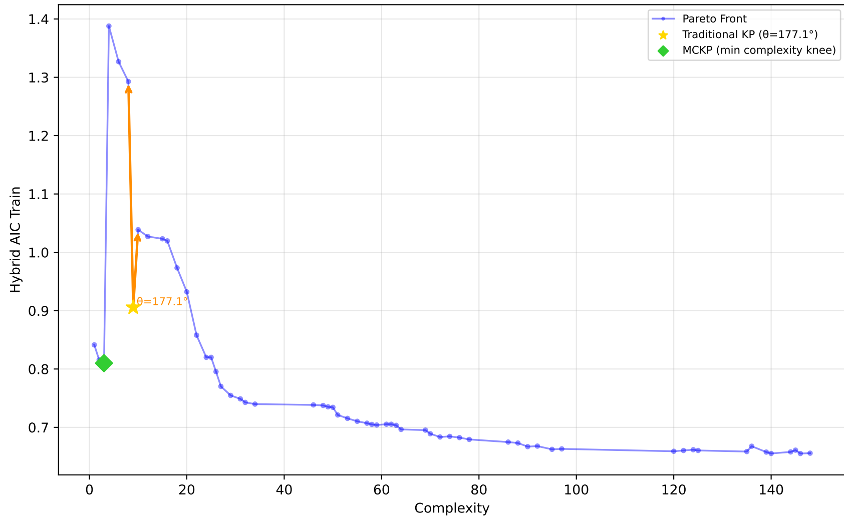
561_cpu - Run 10 - SVP - Hybrid AIC Train \lambda_1=1.00, \lambda_2=0.00, \lambda_3=0.40 | Difficulty: 1.00 | Method: hmr
