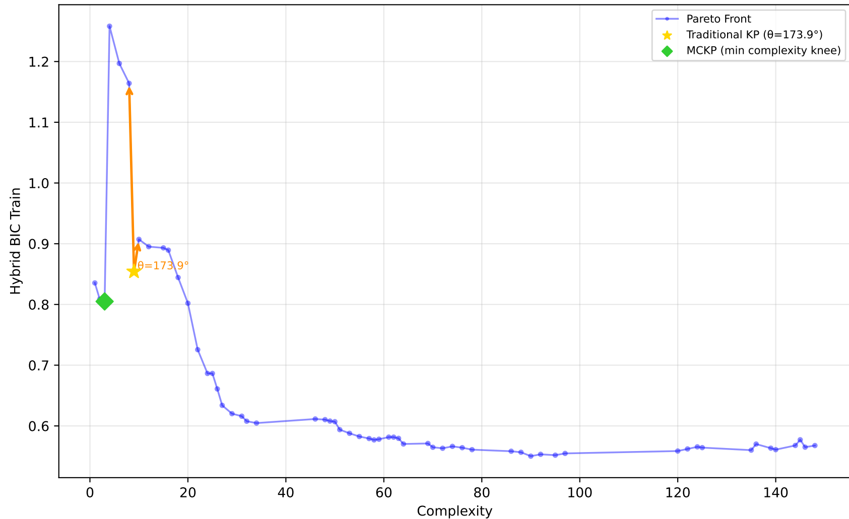
561_cpu - Run 10 - SVP - Hybrid BIC Train \lambda_1=0.90, \lambda_2=0.00, \lambda_3=0.30 | Difficulty: 1.00 | Method: hmr
