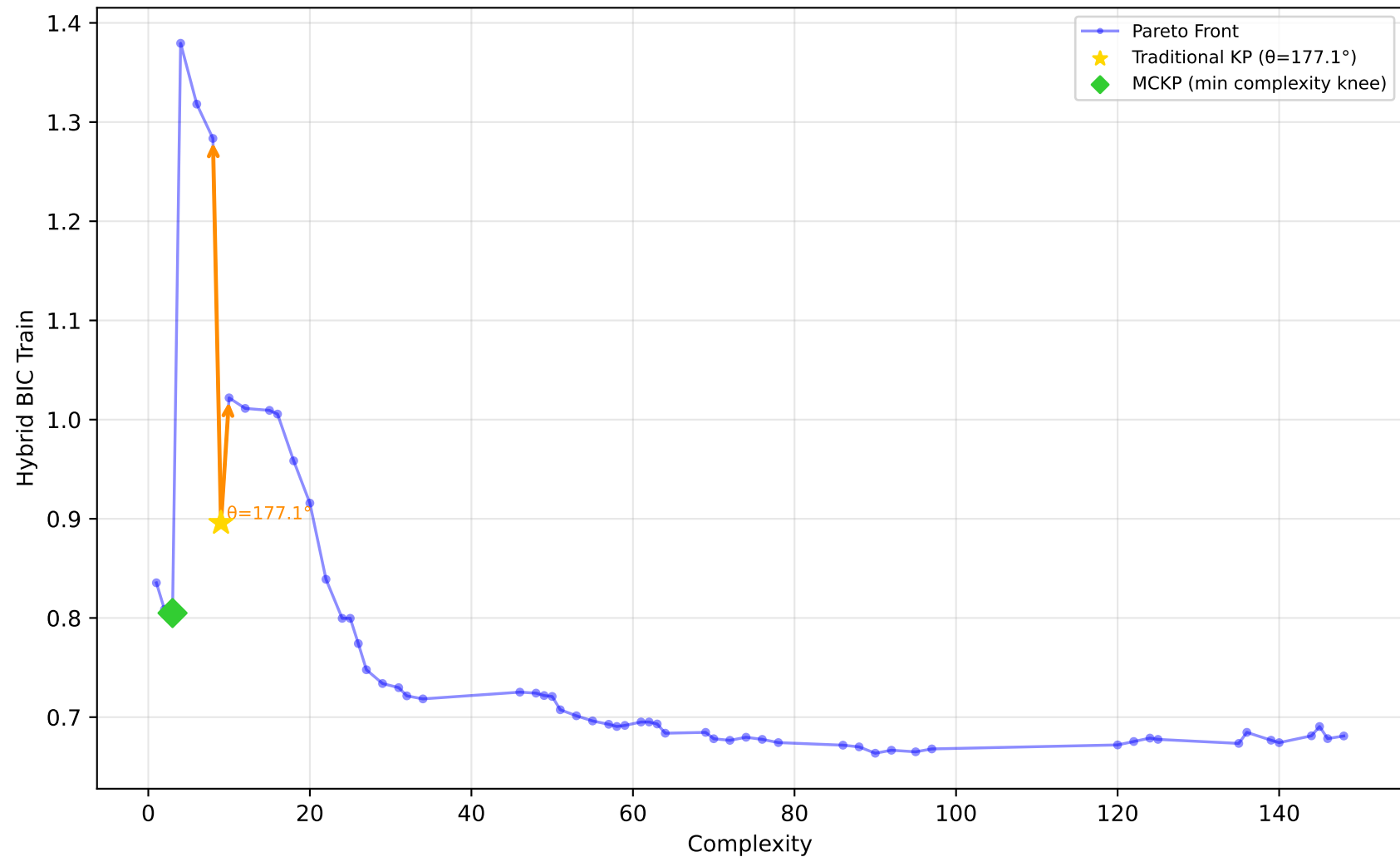
561_cpu - Run 10 - SVP - Hybrid BIC Train \lambda_1=1.00, \lambda_2=0.00, \lambda_3=0.40 | Difficulty: 1.00 | Method: hmr
