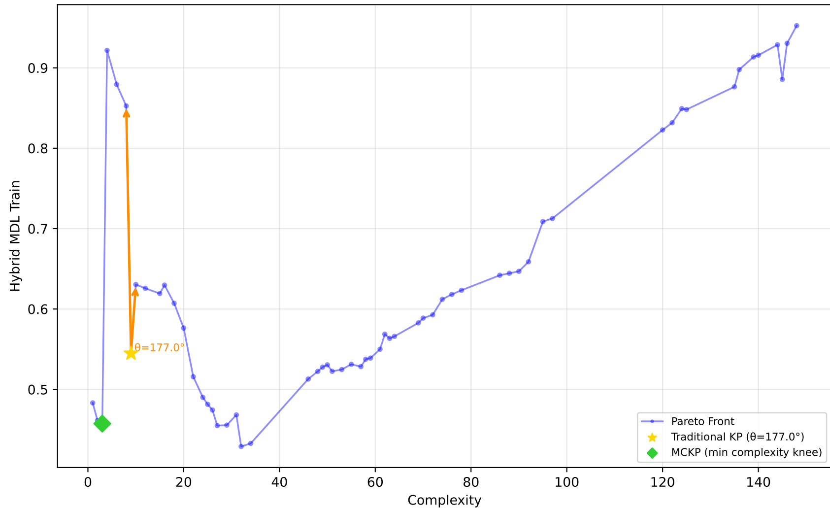
561_cpu - Run 10 - SVP - Hybrid MDL Train \lambda_1=0.90, \lambda_2=0.00, \lambda_3=0.30 | Difficulty: 1.00 | Method: hmr
