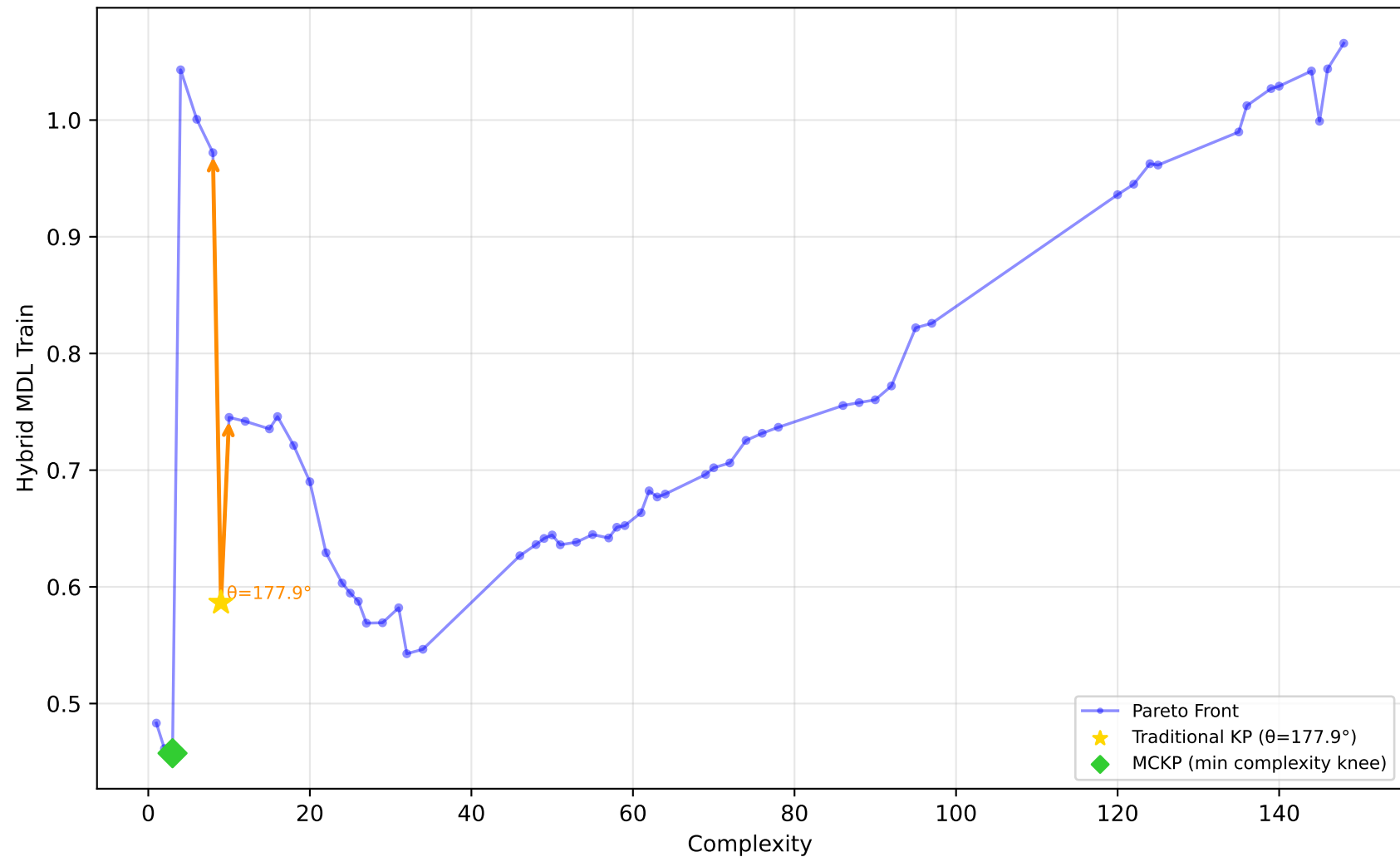
561_cpu - Run 10 - SVP - Hybrid MDL Train \lambda_1=1.00, \lambda_2=0.00, \lambda_3=0.40 | Difficulty: 1.00 | Method: hmr
