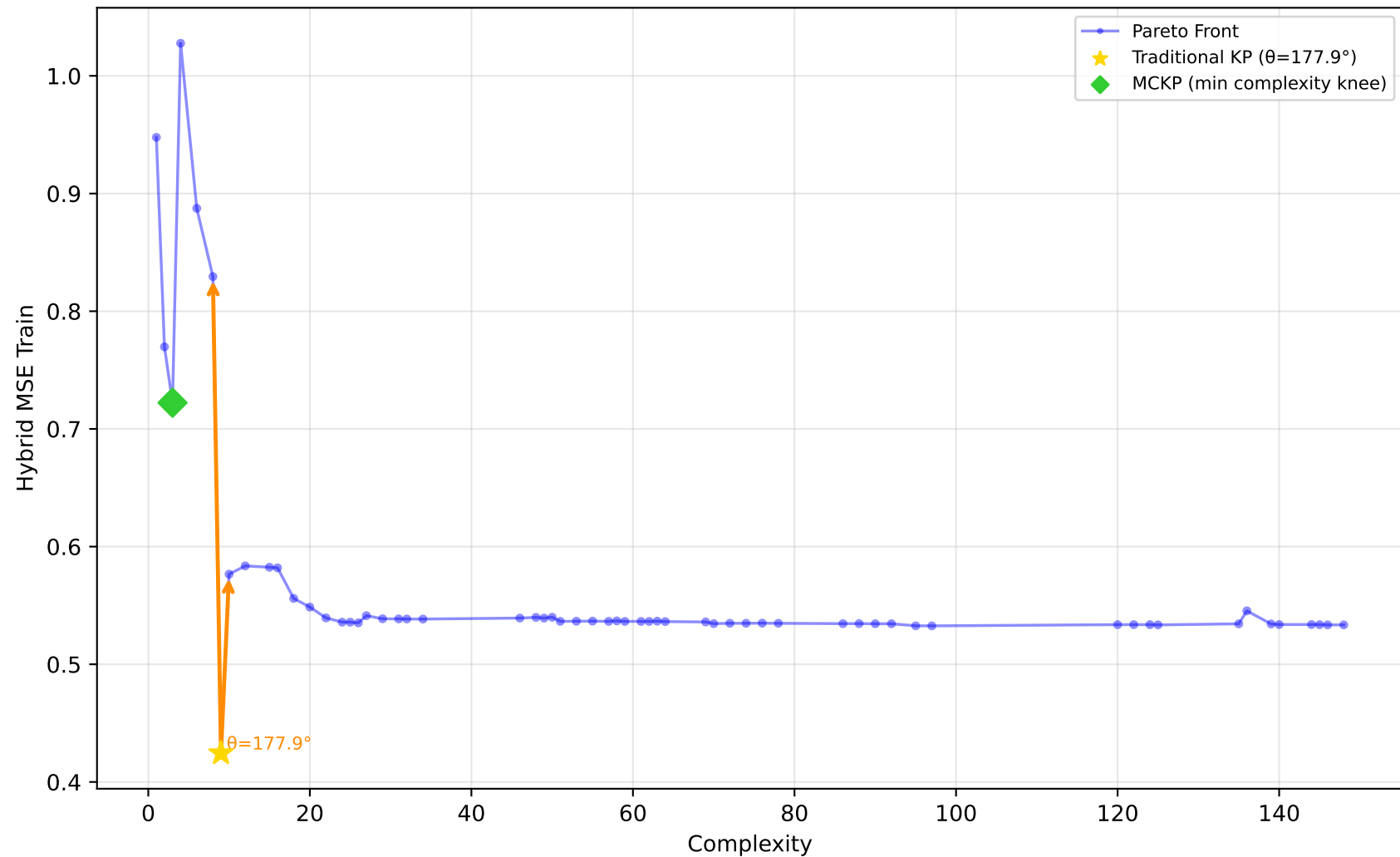
561_cpu - Run 10 - SVP - Hybrid MSE Train \lambda_1=1.00, \lambda_2=0.00, \lambda_3=0.40 | Difficulty: 1.00 | Method: hmr
