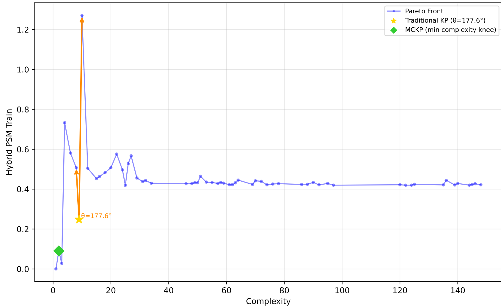
561_cpu - Run 10 - SVP - Hybrid PSM Train \lambda_1=0.90, \lambda_2=0.00, \lambda_3=0.30 | Difficulty: 1.00 | Method: hmr
