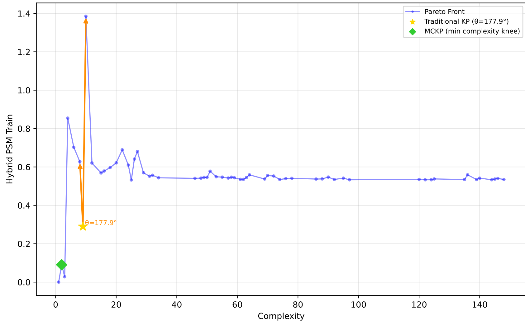
561_cpu - Run 10 - SVP - Hybrid PSM Train \lambda_1=1.00, \lambda_2=0.00, \lambda_3=0.40 | Difficulty: 1.00 | Method: hmr
