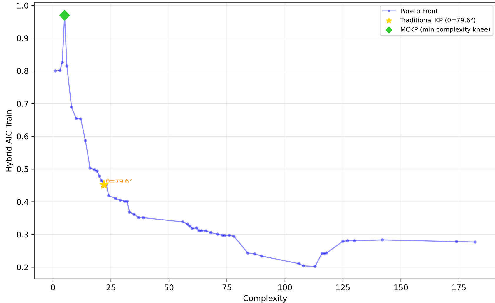
561_cpu - Run 11 - MVP - Hybrid AIC Train \lambda_1=0.50, \lambda_2=0.20, \lambda_3=0.00 | Difficulty: 1.00 | Method: hmr
