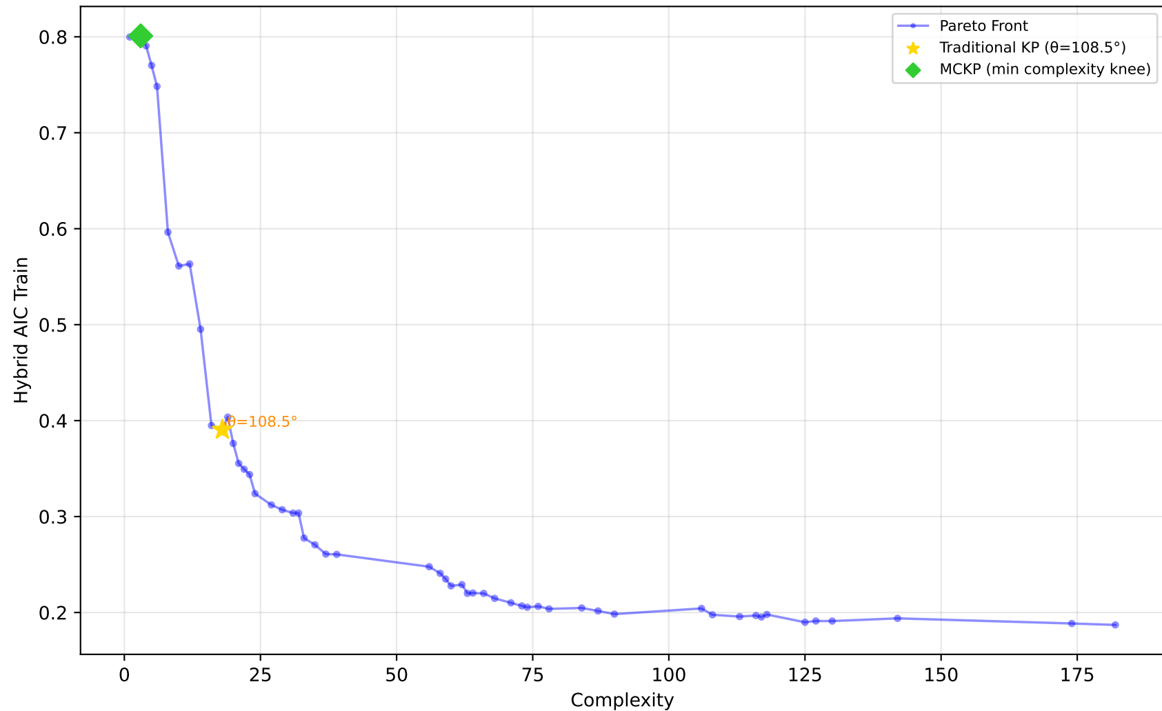
561_cpu - Run 11 - MVP - Hybrid AIC Train \lambda_1=0.70, \lambda_2=0.00, \lambda_3=0.10 | Difficulty: 1.00 | Method: hmr
