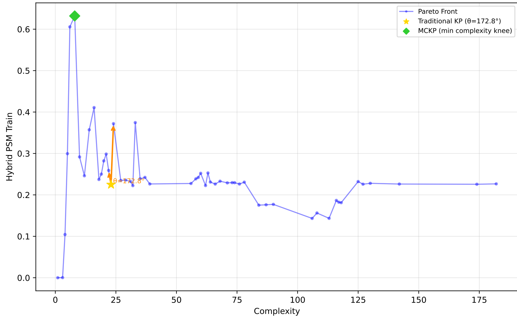
561_cpu - Run 11 - MVP - Hybrid PSM Train \lambda_1=0.50, \lambda_2=0.20, \lambda_3=0.00 | Difficulty: 1.00 | Method: hmr
