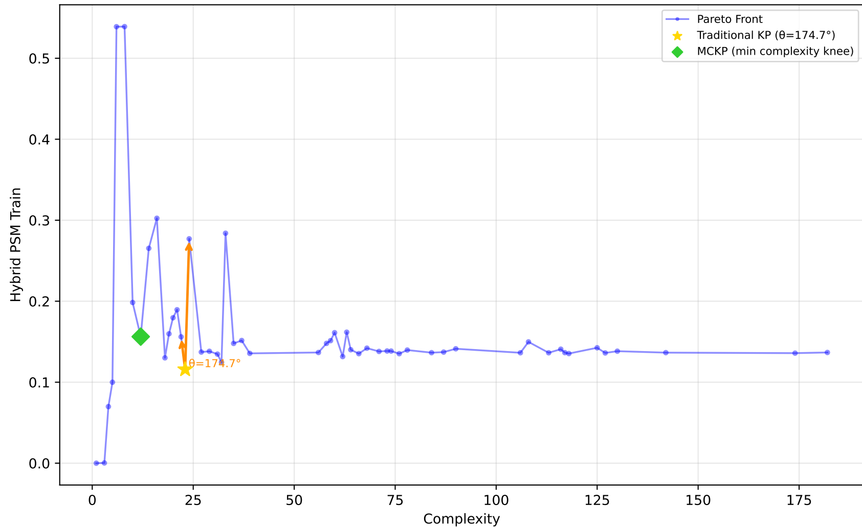
561_cpu - Run 11 - MVP - Hybrid PSM Train \lambda_1=0.70, \lambda_2=0.00, \lambda_3=0.10 | Difficulty: 1.00 | Method: hmr
