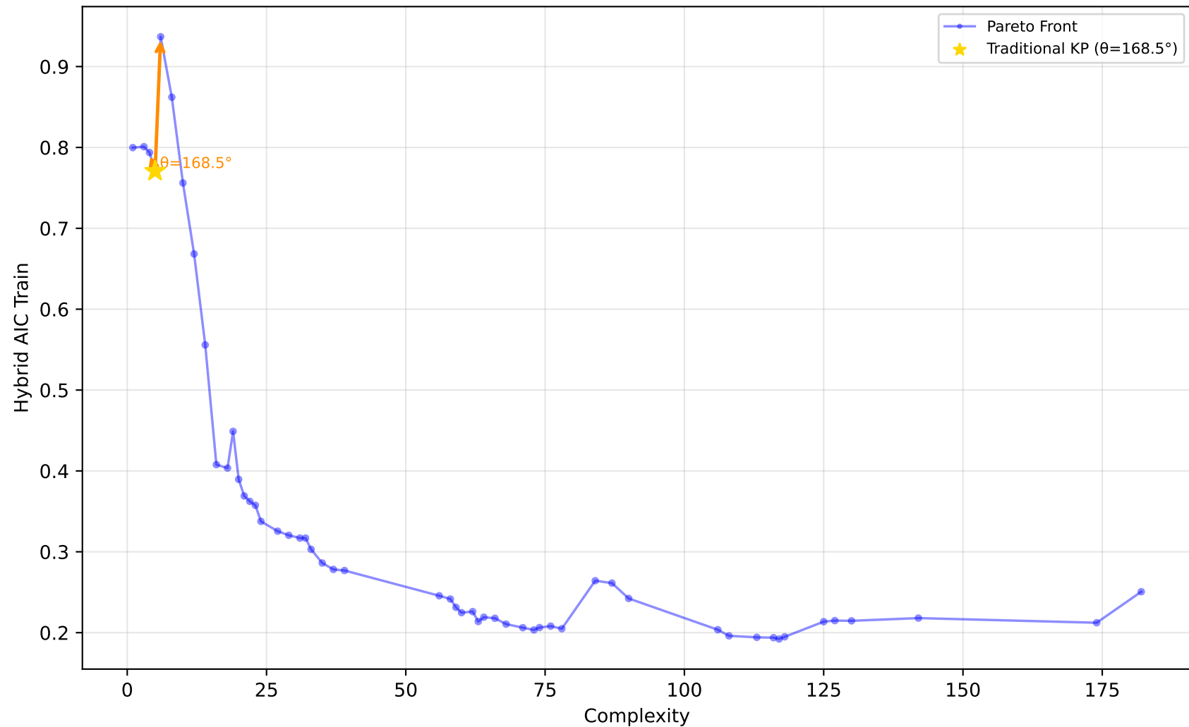
561_cpu - Run 11 - SVP - Hybrid AIC Train \lambda_1=1.00, \lambda_2=0.00, \lambda_3=0.40 | Difficulty: 1.00 | Method: hmr
